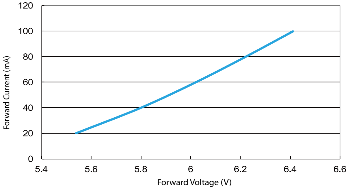
Forward Current vs. Forward Voltage for PLCC 2835 0.4W series
