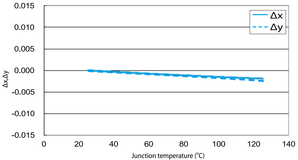
\Delta x, \Delta y vs. Junction temperature for PLCC 2835 0.4W Series
