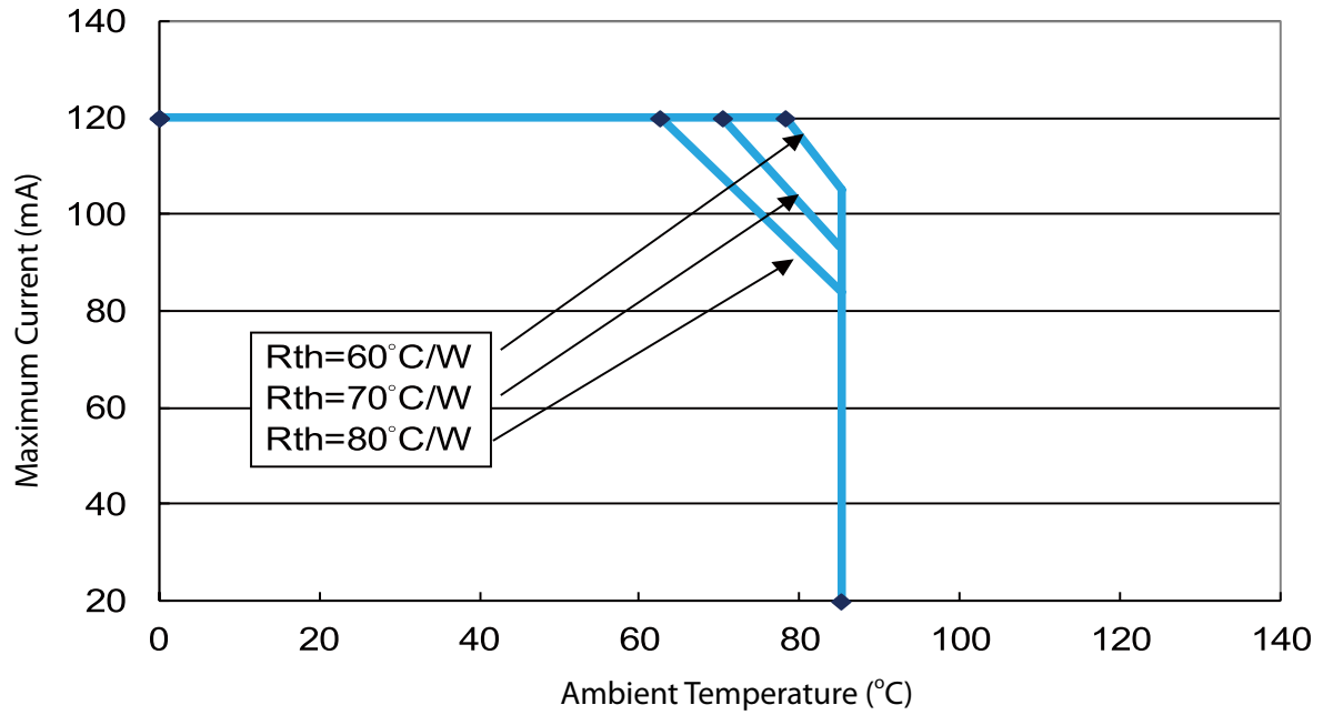
Maximum Current vs. Ambient Temperature for PLCC 2835 0.4W series
