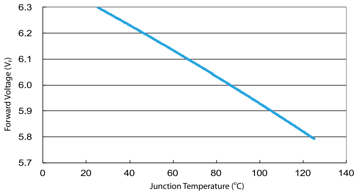
Forward voltage vs. junction temperature for PLCC 2835 0.4W series
