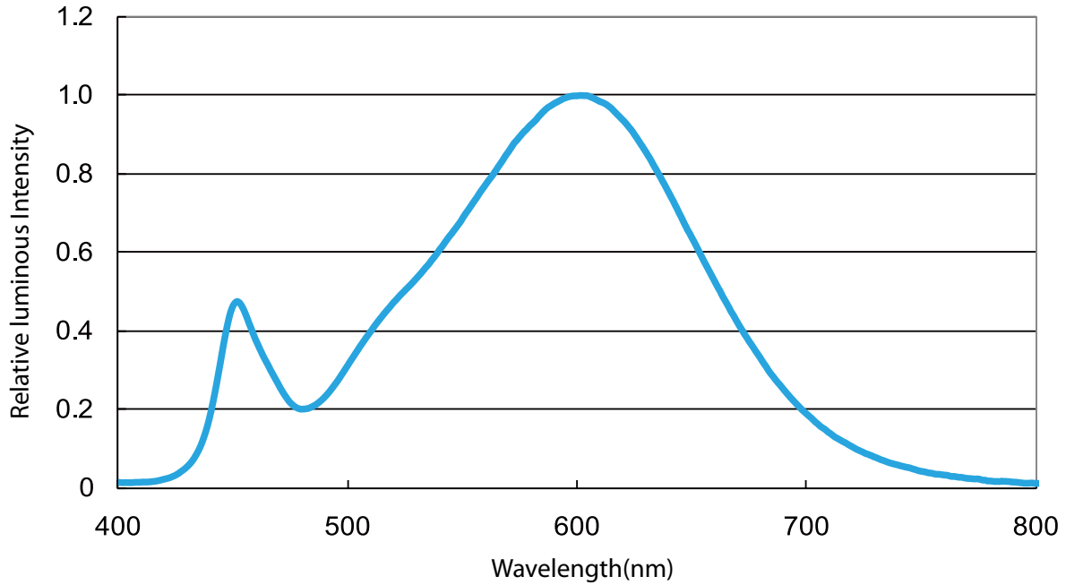
Color Spectrum at a typical CCT for PLCC 2835 0.4W series
