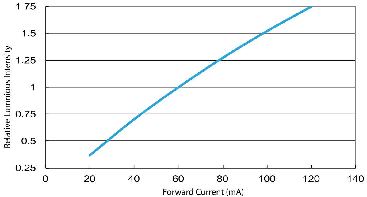
Luminous Intensity vs. Forward Current for PLCC 2835 0.4W series
