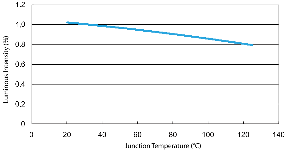
Luminous flux vs. junction temperature for PLCC 2835 0.4W series
