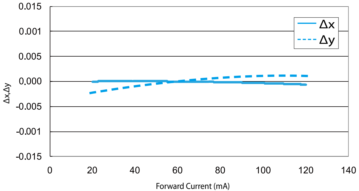
\Delta x, \Delta y vs. Forward Current for PLCC 2835 0.4W Series
