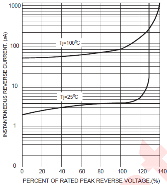
FIG.3-TYPICAL REVERSE CHARACTERISTICS
