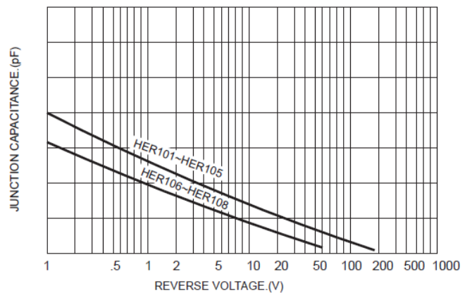
FIG.6-TYPICAL JUNCTION CHARACTERISTICS
