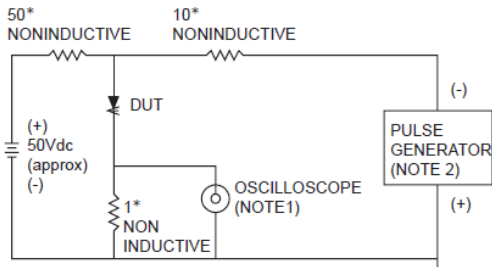
FIG.1- REVERSE RECOVER TIME CHARACTERISTIC AND TEST CIRCUIT DIAGRAM
