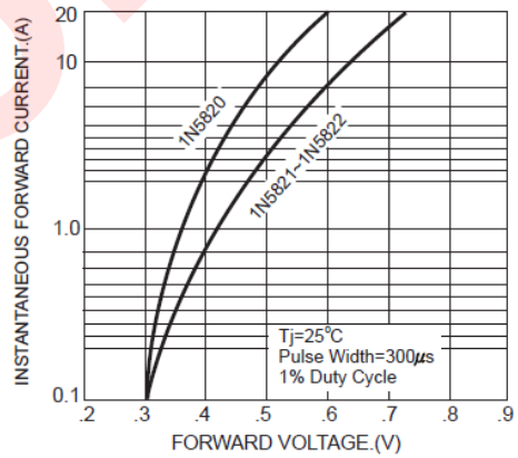
FIG.4-TYPICAL FORWARD CHARACTERISTICS
