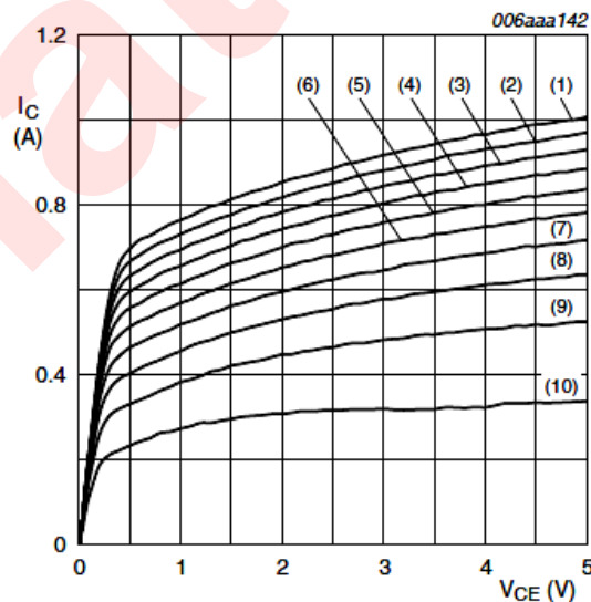
Fig 12. Selection -40: Collector current as a function of collector-emitter voltage; typical values
