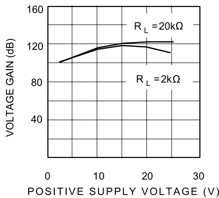
Figure 14: Voltage gain
