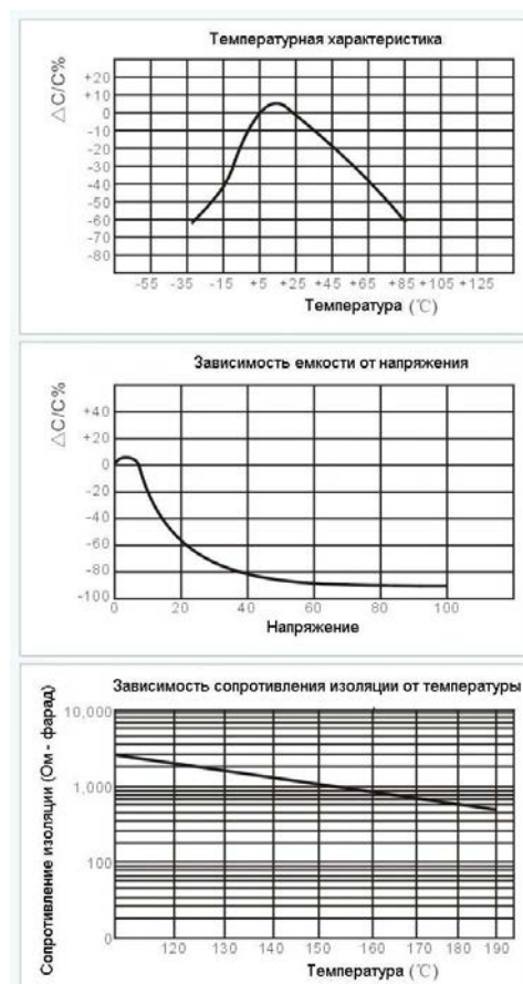
Y5V
