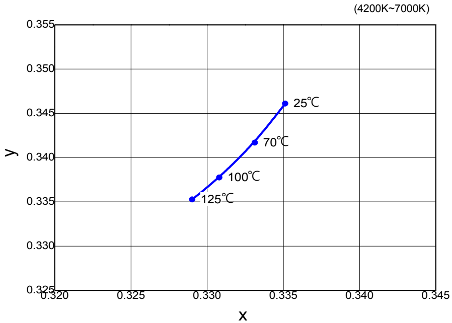
Fig 8. Chromaticity Coordinate vs. Junction Temperature, I_F = 200\text{mA}
