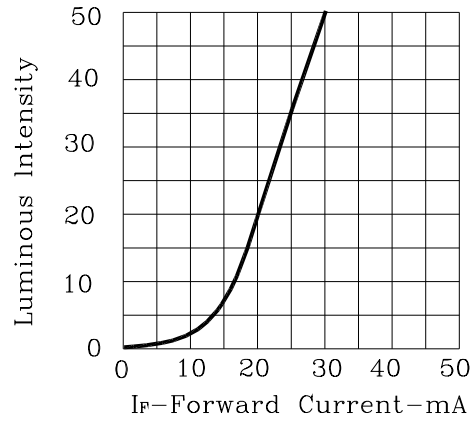
Luminous Intensity VS. Forward Current (mcd)
