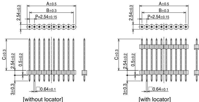
●Board Through-hole Diameter : \phi 1.0^{+0.1}
