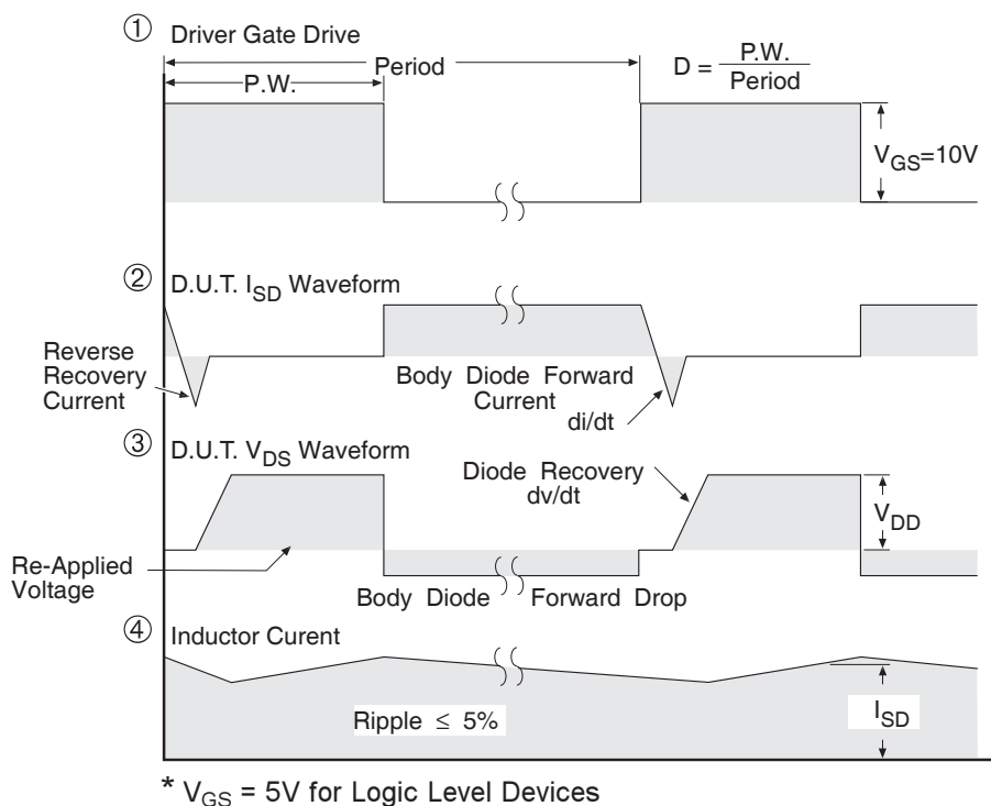
Fig 12. For N-Channel HEXFETS
