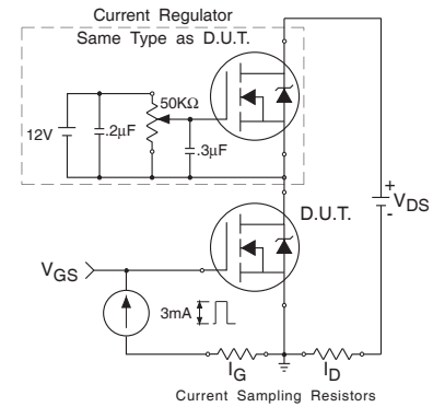
Fig 9b. Gate Charge Test Circuit
