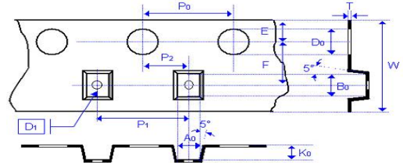
Fig. 8.2 The dimension of plastic tape
