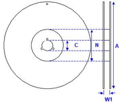
Fig. 8.3 The dimension of reel
