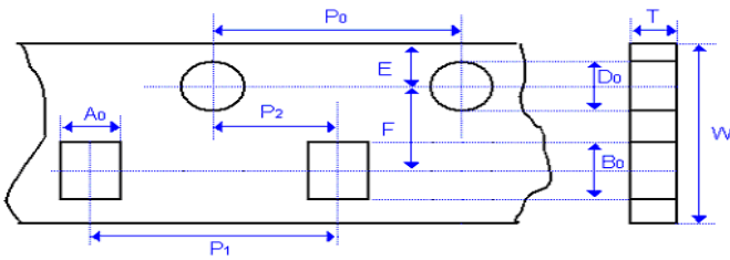
Fig. 8.1 The dimension of paper tape
