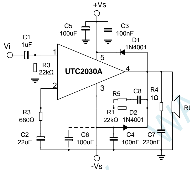
Fig. 13 Typical amplifier with split power supply
