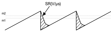
Fig.19 20kHz sawtooth waveform
