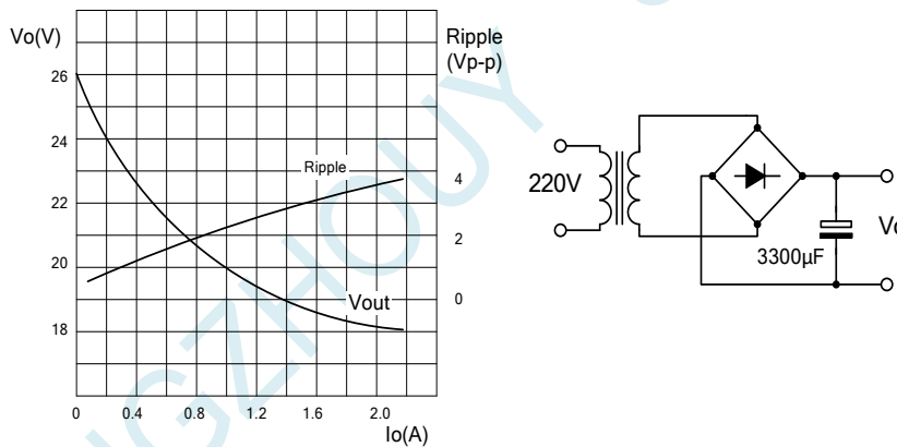
Fig.23 DC characteristics of 50W non-regulated supply
