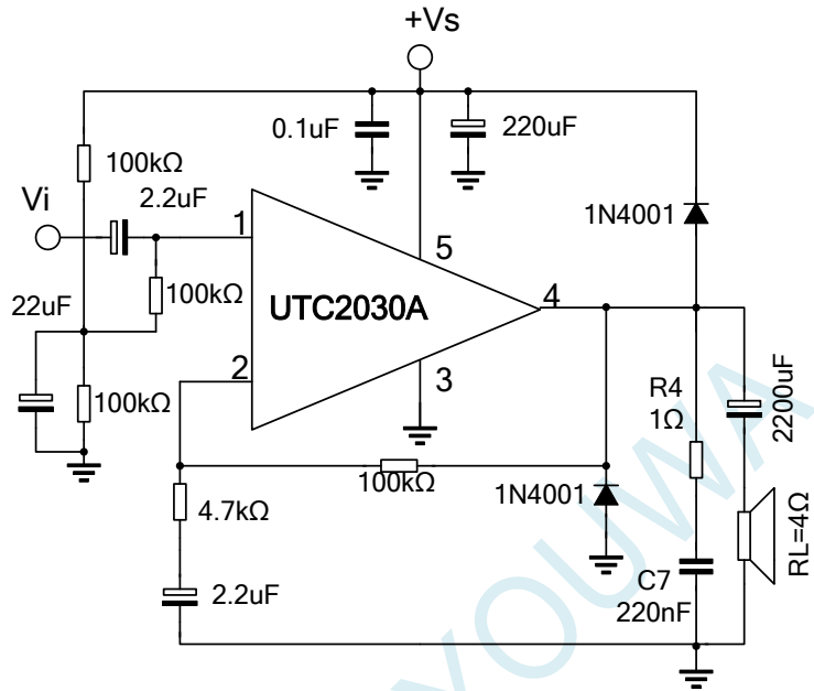
Fig. 1 Single supply amplifier
