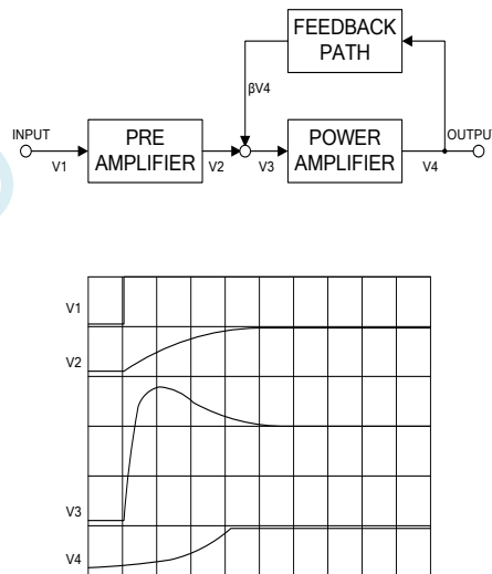
Fig.18 Overshoot phenomenon in feedback amplifiers
