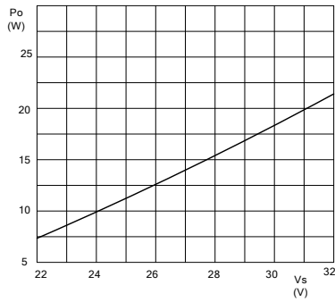
Fig. 9 Output power vs. supply voltage
