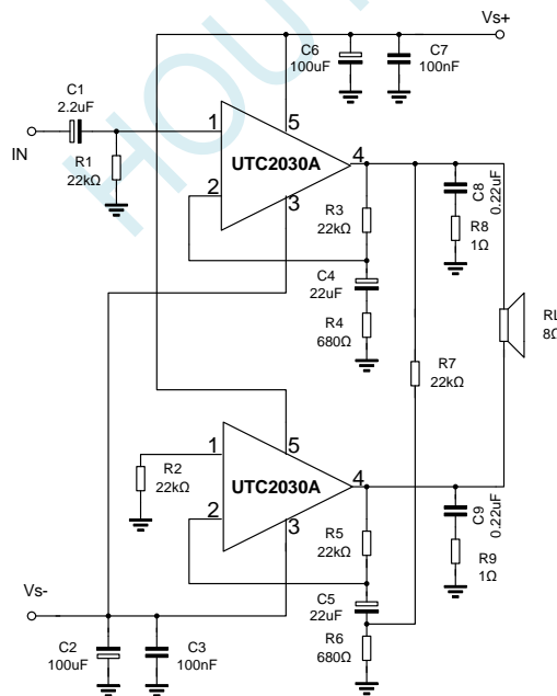
Fig. 14 Bridge amplifier with split power supply( P_o=34W, V_s+=16V, V_s-=16V )
