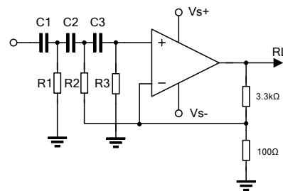
Fig. 16 Active power filter
