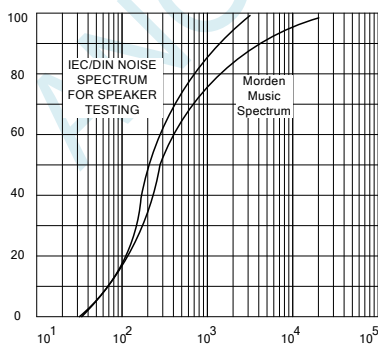
Fig. 15 Power distribution vs. frequency
