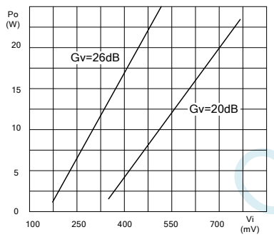
Fig. 11 Output power vs. Input level
