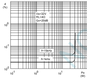
Fig. 10 Total harmonic distortion vs. output power
