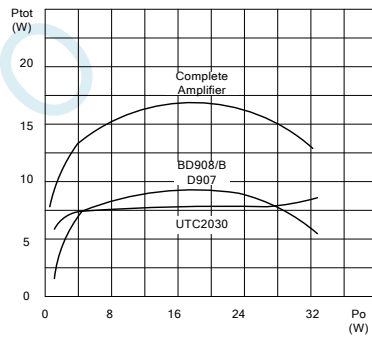
Fig. 12 Power dissipation vs. output power
