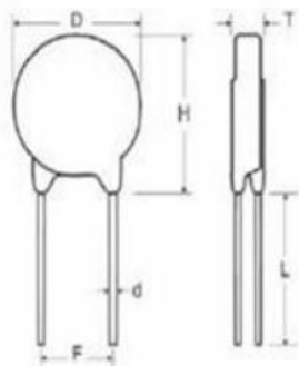
S Type(Straight Lead)
