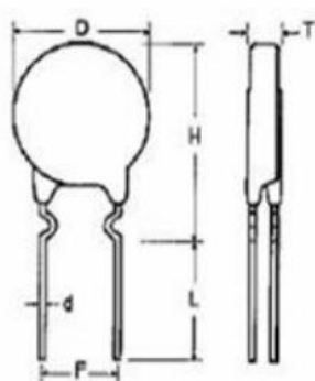
I Type(Inner Crimped Lead)
