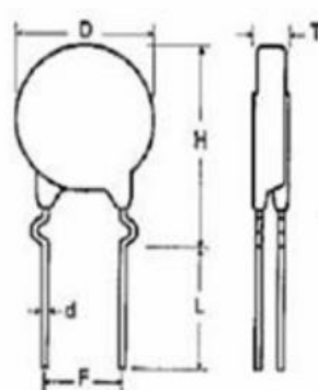
C Type(Out Crimped Lead)
